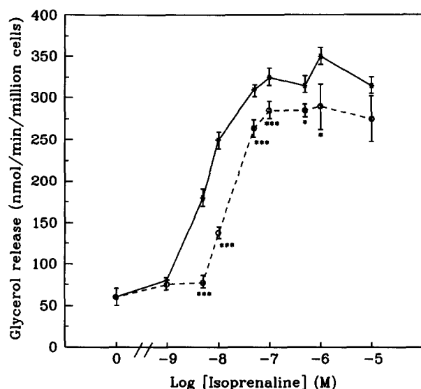
Fig. 2. Effect of AICAR on lipolysis stimulated by isoprenaline in primary adipocytes. Adipocytes were incubated for 60 min in control experiments (*) or with 500 \mu M AICAR (○) prior to a challenge with isoprenaline. The data points represent the mean of three separate cell incubations. The standard deviations from the mean are indicated by the vertical bars. The statistical significance of differences, as determined by a two-tailed t -test, is indicated (*** P < 0.001, * P < 0.01).
